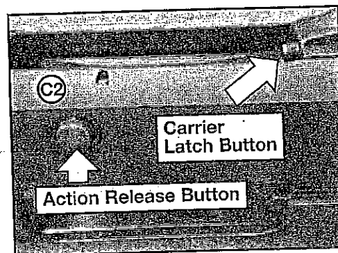
Incorrect - Action may close. The carrier latch button is fully extended indicating it has not been properly depressed to lock the action open.
