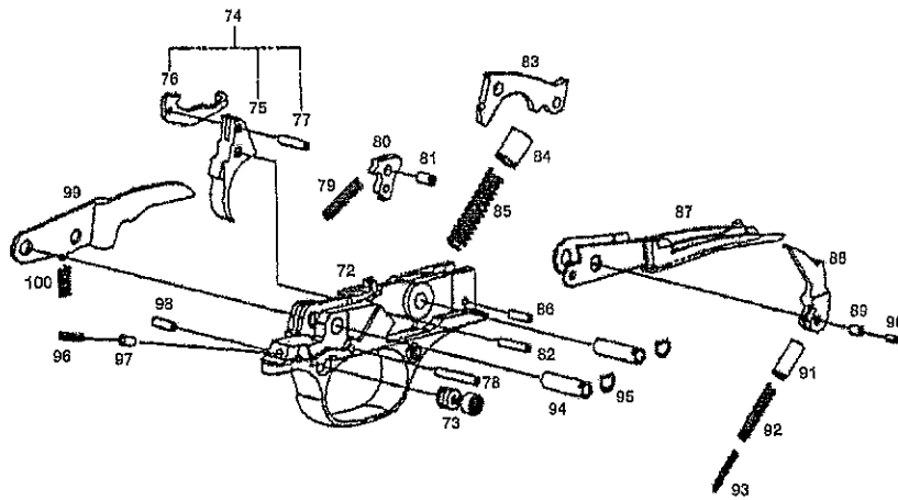
Figure 2: Trigger Plate Parts Assembly
